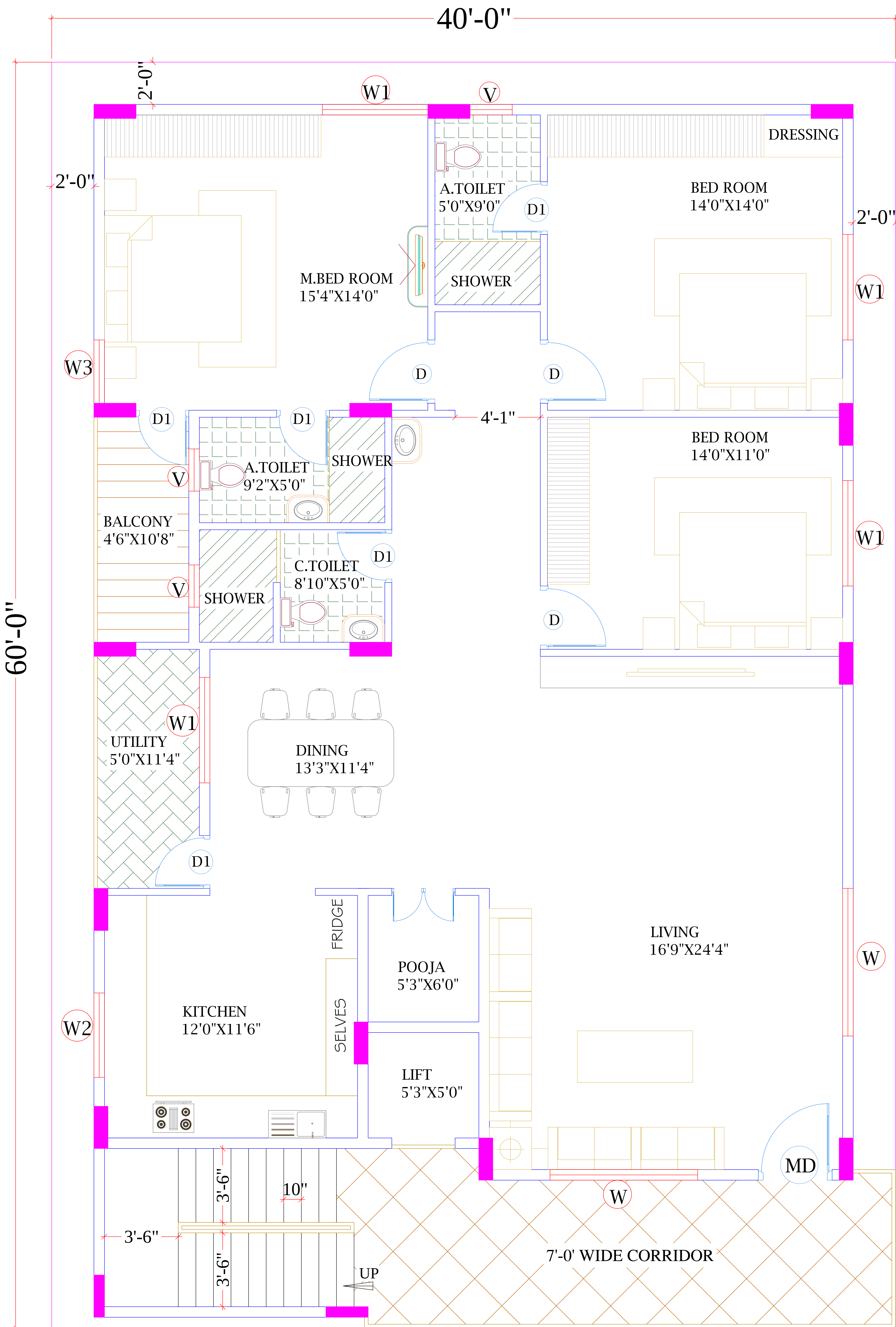
E A S T B Y R O A D TYPICAL FLOOR PLAN(G.F,1st.F&2nd.F)
